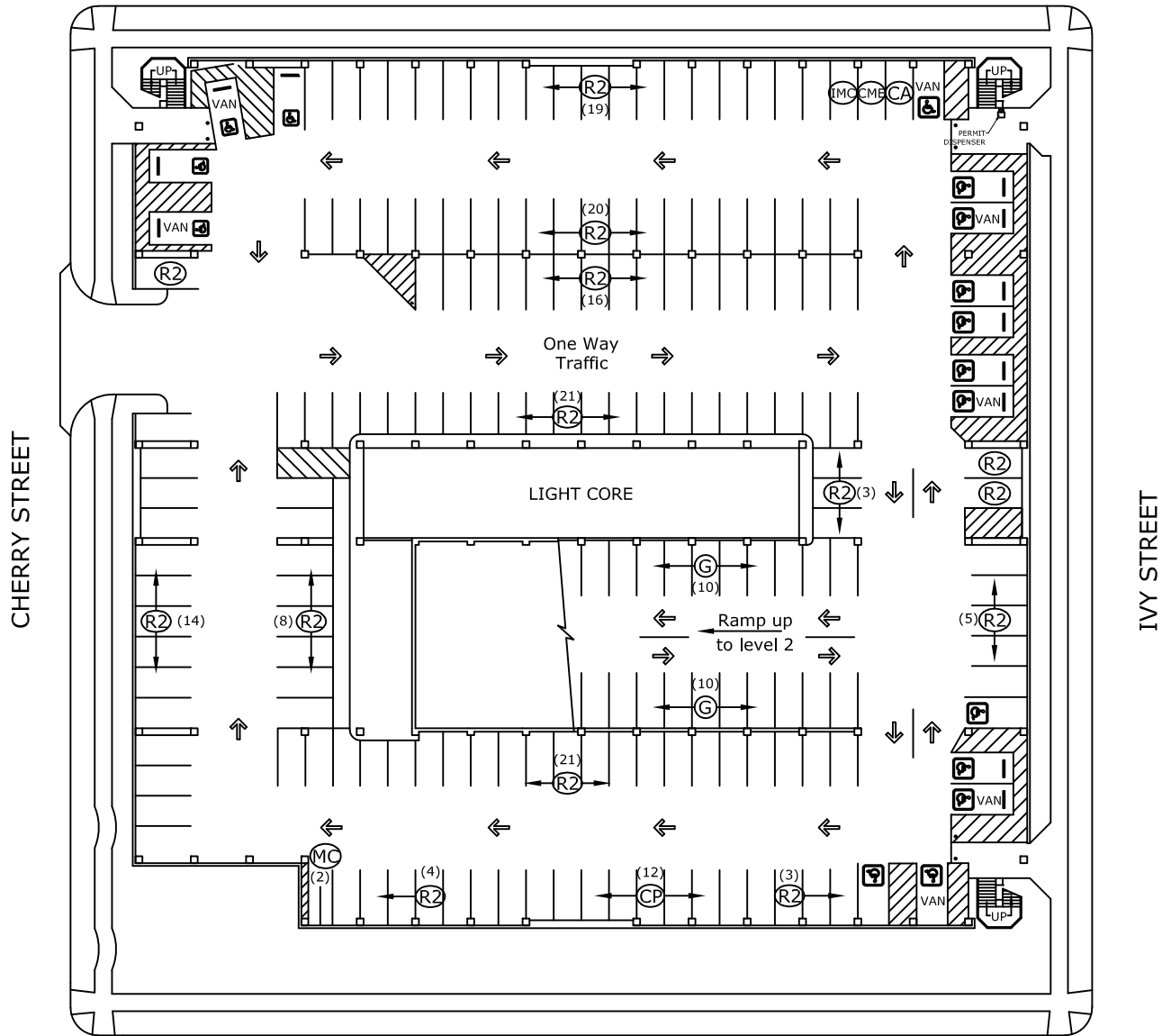
PARKING STRUCTURE STALL COUNT
