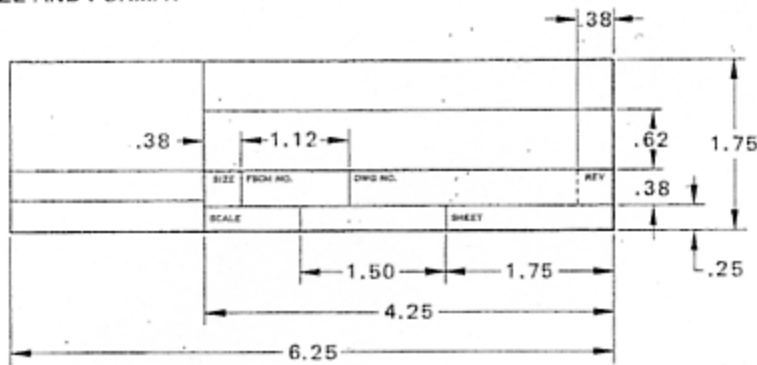
NOTE: All dimensions are in inches. 1 inch = 25.4 mm. FIG. 4(a) TITLE BLOCK FOR A, B, C, AND G - SIZES
