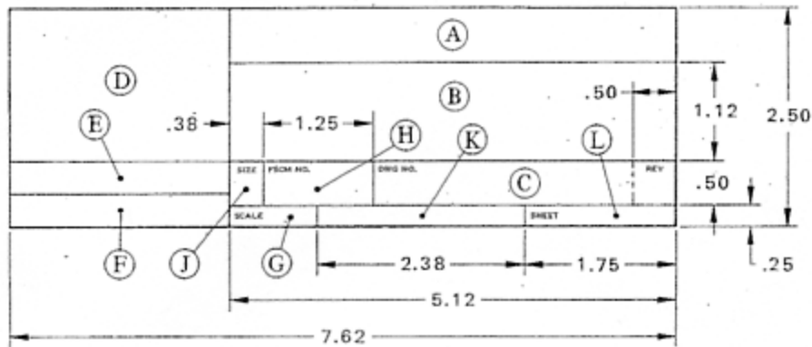
NOTE: All dimensions are in inches. 1 inch = 25.4 mm. FIG. 4(b) TITLE BLOCK FOR D, E, F, H, J, AND K - SIZES
