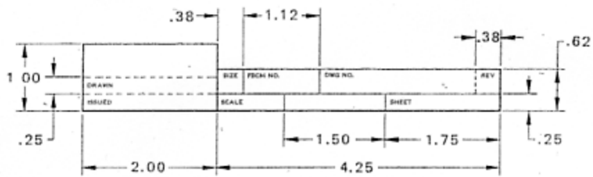
NOTE: All dimensions are in inches. 1 inch = 25.4 mm. FIG. 5(a) CONTINUATION SHEET TITLE BLOCK FOR A, B, C, and G - SIZES
