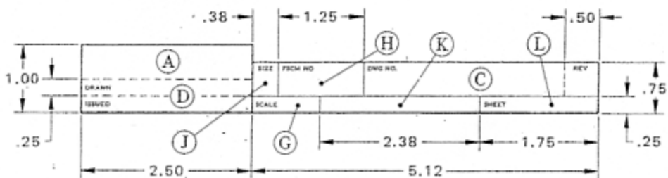
NOTE: All dimensions are in inches. 1 inch = 25.4 mm. FIG. 5(b) CONTINUATION SHEET TITLE BLOCK FOR D, E, F, H, J, AND K - SIZES
